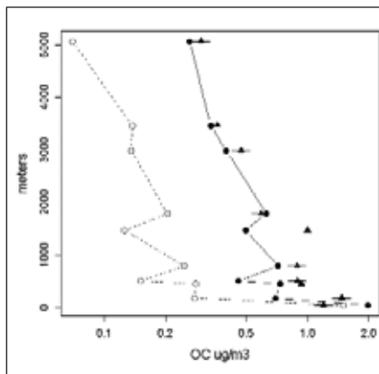
Figure 1. Layer-averaged vertical profiles of modeled and observed organic carbon (OC) on August 14, 2004. Note: Dashed line and "o" indicates layer-averaged base CMAQ OC prediction. Solid line and "•" indicates CMAQ OC prediction with cloud-produced SOA included. OC observations "▲" are based on the International Consortium for Atmospheric Research on Transport and Transformation (ICARTT) New England Air Quality Study - Intercontinental Transport and Chemical Transformation (from Carlton et al.5). The x-axis is log scale.
