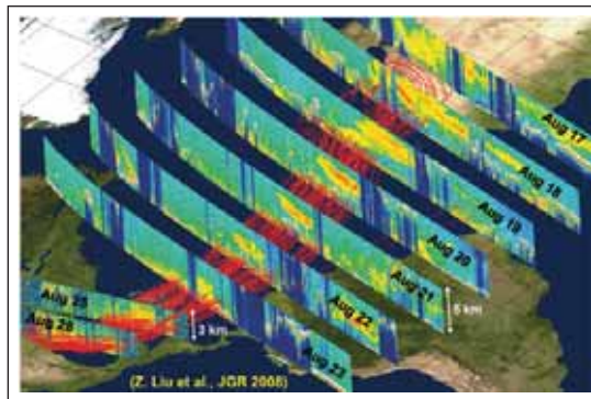
Figure 2. Four-dimensional observations from the CALIPSO satellite lidar measurement sequences of August, 2006 show African dust transport across the Atlantic Ocean (Source: Liu et al.) 9
