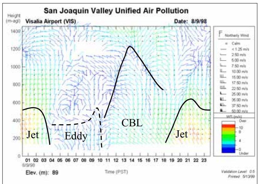
Figure 4. Radar wind profiler data at Visalia on August 9, 1998, showing the nocturnal jet, convective boundary layer (CBL), and eddy flow. This wind pattern was observed on the majority of the episode days.
