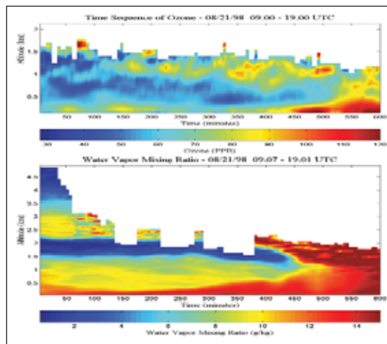
Figure 3. Time sequences of the PBL vertical profiles of water vapor and ozone measured by a Raman lidar at the NARSTO-NEOPS field site in Philadelphia during August 21, 1998. 10
